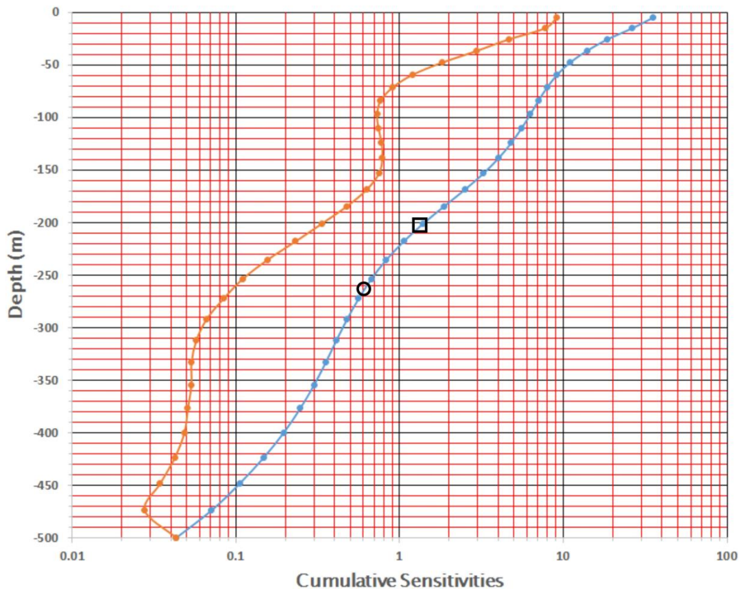
Figure 4. Example of exported sensitivities (orange line) from the GERDA database and the calculated cumulative sensitivities (blue line). Depths, in meters, are on the vertical axis. The horizontal axis is in dimensionless units of cumulative sensitivity. The black square is the location at which the cumulative sensitivity is 1.2 leading to a DOI of approximately 208 m depth. The black circle is the location at which the cumulative sensitivity is 0.6 leading to a DOI of approximately 263 m depth. DOI's for cumulative sensitivity thresholds 1.2 and 0.6 are included in the exported Workbench inversion results xyz file per the inversion configuration setup file.
