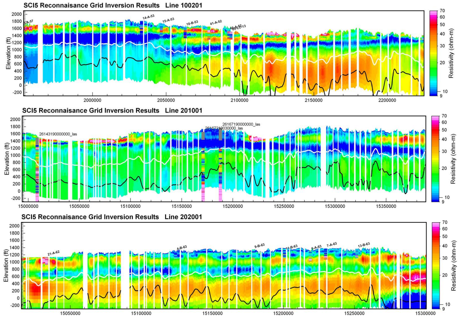
Figure 9. Aarhus Workbench SCI inversion results with DOI's based on cumulative sensitivity thresholds 0.6 (solid white line) and 0.1 (black line) and available borehole resistivity logs from the Nebraska CSD (2014) and the NOGC (2015). Elevation and distance units are in feet.
