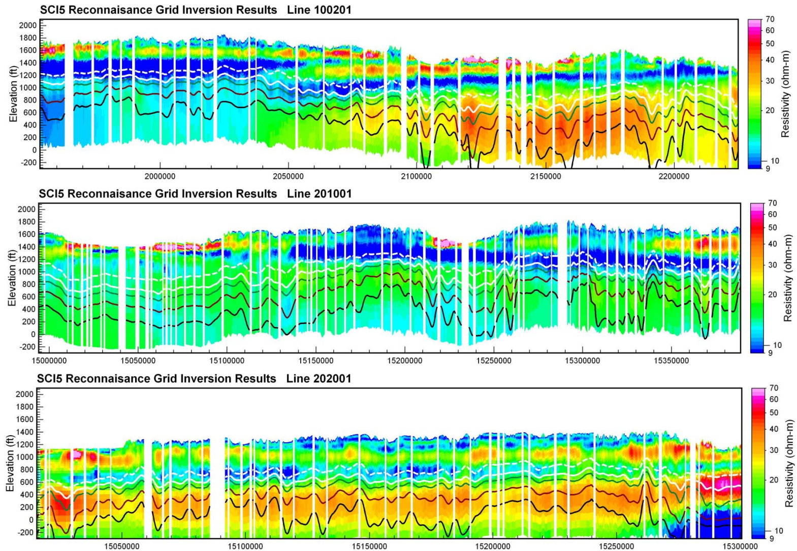
Figure 8. Aarhus Workbench SCI inversion results with DOI's based on cumulative sensitivity thresholds 1.2 (dashed white line), 0.6 (solid white line), 0.4 (green line), 0.2 (brown line), and 0.1 (black line). Elevation and distance units are in feet.
