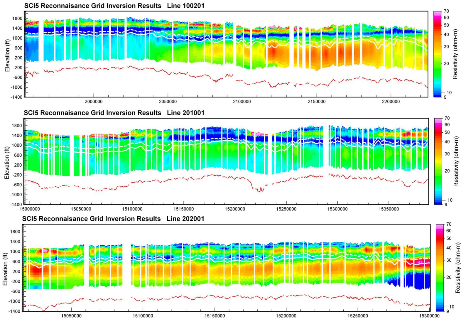
Figure 6. Aarhus Workbench SCI inversion results with the “default” upper and lower DOI’s per Figure 5 plus the theoretical DOI (red line) based on equation (5) using a 0.5 nV/m 2 noise level. Elevation and distance units are in feet.
