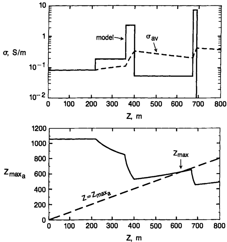
Figure 1. Illustration of the inverse relationship between changes in resistivity (the inverse of the conductivity s ) and theoretical depth of investigation (from Spies, 1989). As the electrical conductivity increases (resistivity decreases) in the top figure, the depth of investigation decreases (bottom figure).
