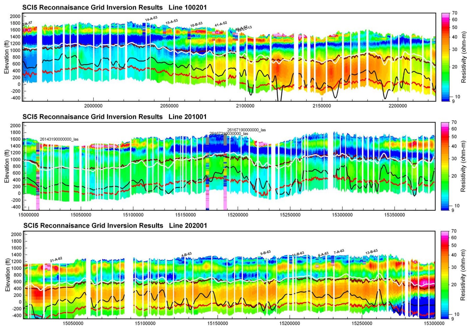
Figure 10. SCl inversion results with DOI's based on cumulative sensitivity thresholds 0.6 (solid white line) and 0.1 (black line), borehole resistivity logs, and theoretical DOIs based on equation (4) using noise levels of 4.0 nV/m 2 (red line) and 150 nV/m 2 (brown line). Elevation and distance units are in feet.
