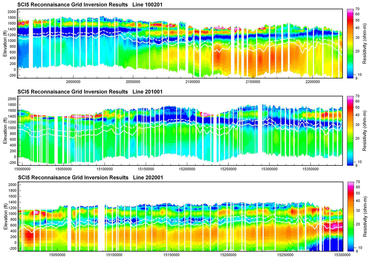
Figure 5. Aarhus Workbench SCI inversion results for west to east (top, left to right) and south to north (bottom & center, left to right) oriented flight lines. The data gaps are where electromagnetic coupling affects have been removed. The dashed lines represent the DOI at a cumulative sensitivity threshold of 1.2 and the solid lines the DOI at a cumulative sensitivity threshold of 0.6. Elevation and distance units are in feet.
