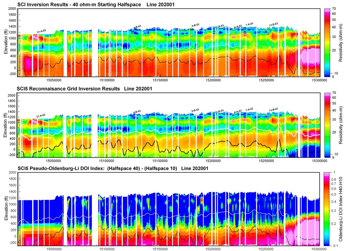
Figure 12. Aarhus Workbench SCI inversion results with DOI's for cumulative sensitivity thresholds 0.6 (solid white line) and 0.1 (black line) and available borehole resistivity logs. Top – 40 ohm-m starting halfspace. Middle – 10 ohm-m starting halfspace. Bottom – Calculated Oldenburg-Li DOI Index (Note that the range is not completely 0 < x < 1 ). Elevation and distance units are in feet.
