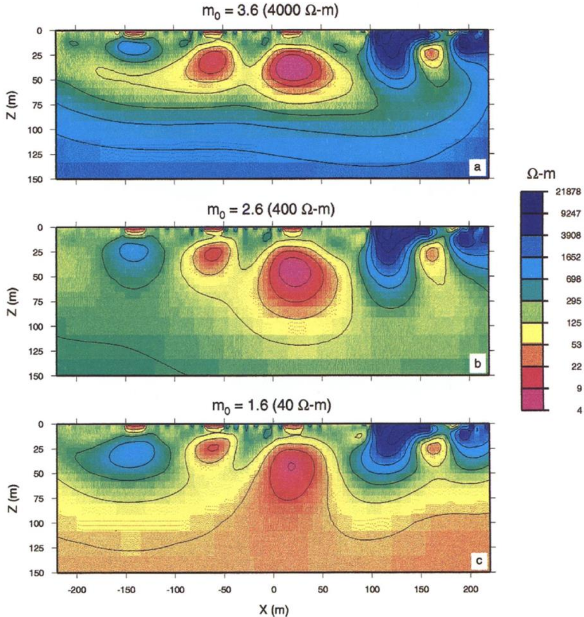
Figure 3. Example from/of Oldenburg–Li (1999) process for determining the DOI. Three inversion runs with very different reference model halfspaces (4000 ohm-m, 400 ohm-m, and 40 ohm-m) produce three models. Where the model results are similar, the inversion features are data-driven. Where the models vary, usually at depth, the
