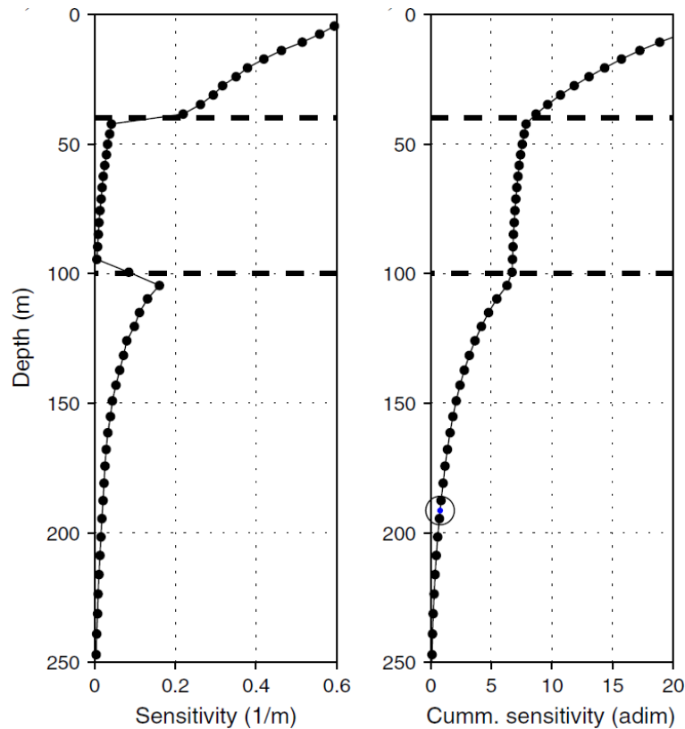
Figure 2. Example sensitivity plots from Christiansen–Auken (2012). Left – Error-, thickness-normalized sensitivity; Right – Cumulative sensitivity plot. The circle indicates the DOI given by a threshold value of 0.8.
