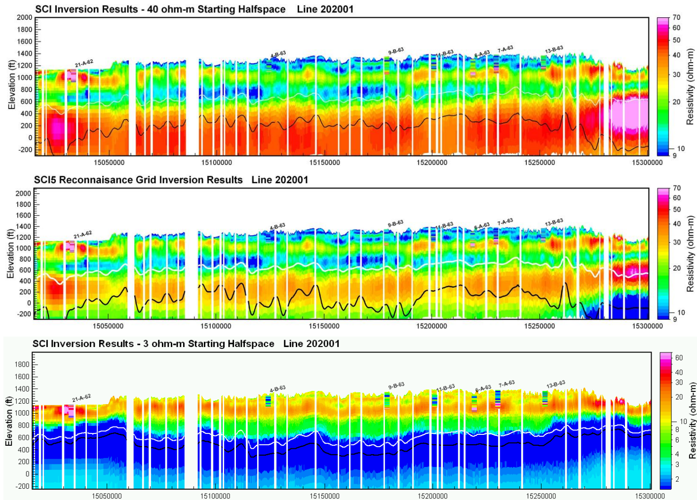
Figure 11. Aarhus Workbench SCI inversion results with DOI's based on cumulative sensitivity thresholds 0.6 (solid white line) and 0.1 (black line) and available borehole resistivity logs from the Nebraska CSD (2014). Top – 40 ohm-m starting halfspace with average Resdata Error = 0.547. Middle – 10 ohm-m starting halfspace (same as in previous figures) with average Resdata Error = 0.539. Bottom – 3 ohm-m starting halfspace with average Resdata Error = 0.799. Elevation and distance units are in feet. The resistivity range is 9–70 ohm-m for all three profiles.
