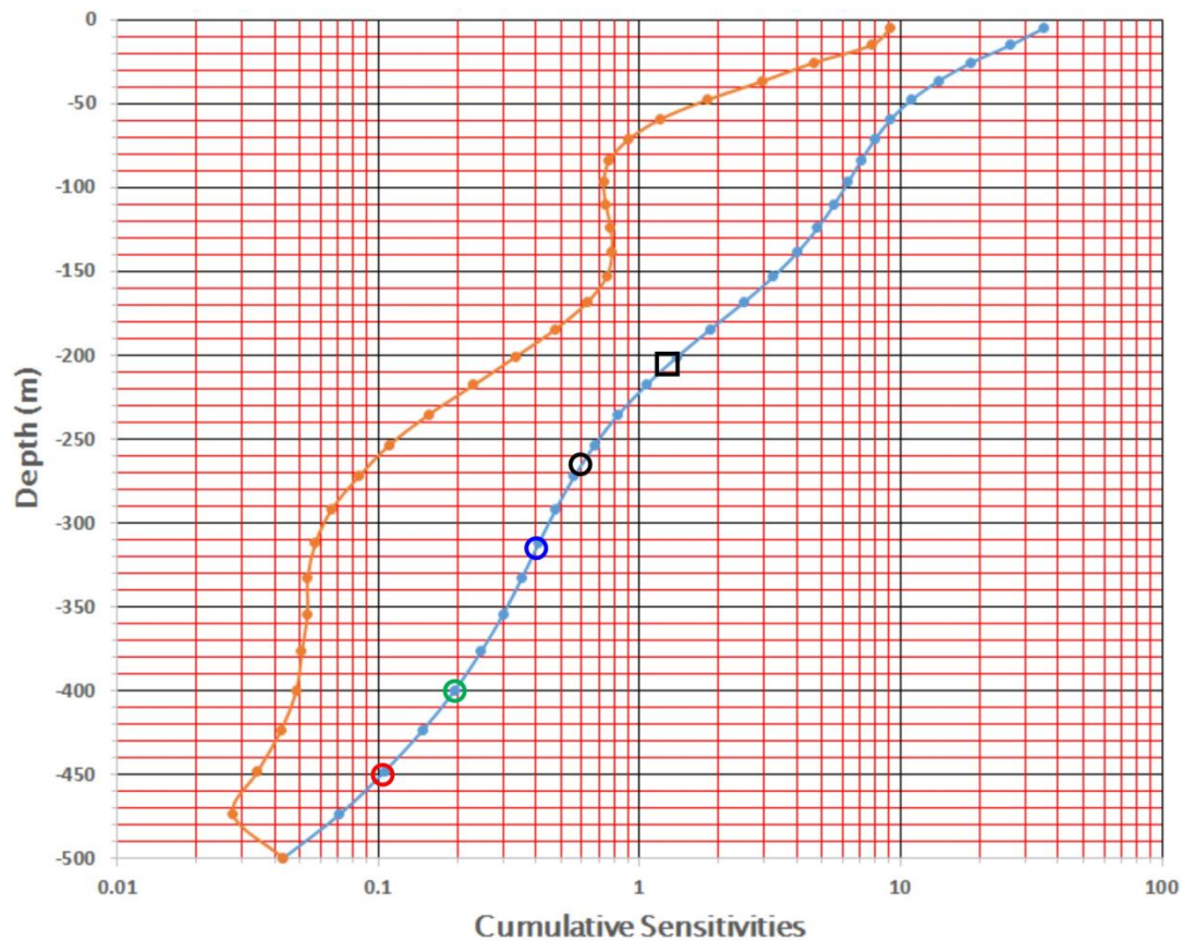
Figure 7. Example of exported sensitivities (orange line) from the GERDA database and the calculated cumulative sensitivities (blue line). Depths in meters are on the vertical axis. The horizontal axis is in units of cumulative sensitivity. The black square is the cumulative sensitivity at 1.2 (DOI ~ 208 m depth); The black circle is the cumulative sensitivity at 0.6 (DOI ~ 262 m depth); The blue circle is the cumulative sensitivity at 0.4 (DOI ~ 309 m depth); The green circle is the cumulative sensitivity at 0.2 (DOI ~ 400 m depth) The red circle is the cumulative sensitivity at 0.1 (DOI ~ 452 m depth).
